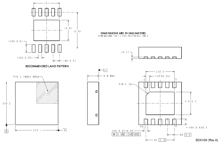
10-Lead LLP Order Numbers DAC082S085C1SD NS Package Number SDA10A
